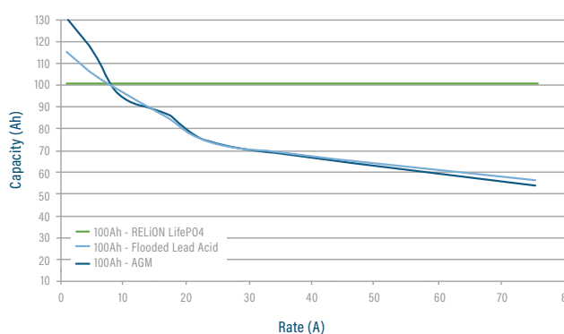
CAPACITY OF RELiON LiFePO4 vs. LEAD ACID at VARIOUS RATES OF DISCHARGE
